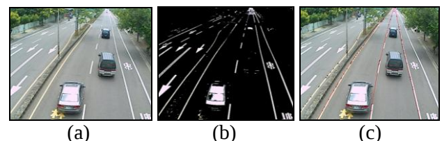
Fig. 4 The demonstration of road lane detection (a) original image (b) color filtering and binarization (c) the detected lane
