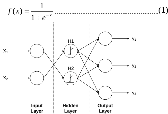
Fig. 5 The model of three-layered back-propagation neural network
