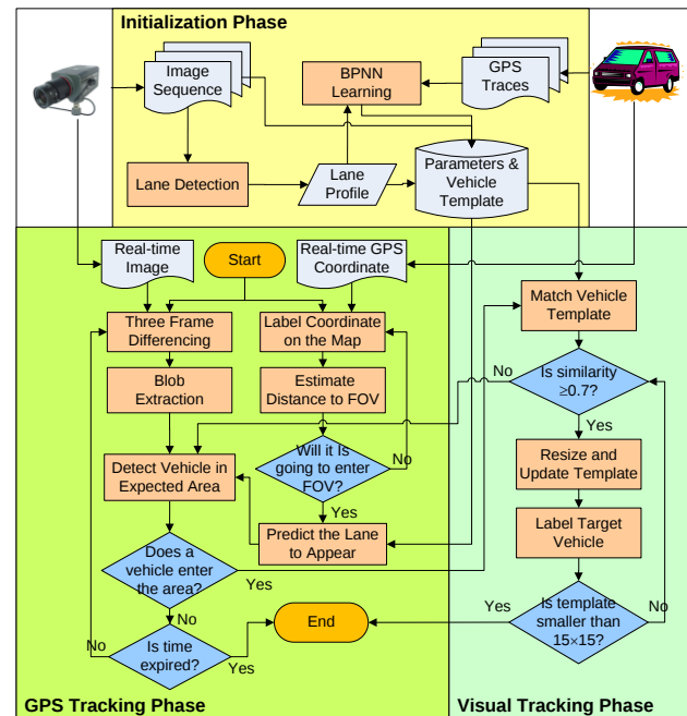
Fig. 3 The operation process of GPS-VT for vehicles
