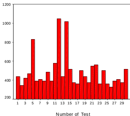
Fig. 2 The transmission delay of GPRS connection
