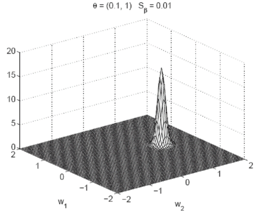
Fig. 2. For multiplicative weight noise case, the conditional probability P(\tilde{\theta}|\theta) for \theta equals to (0.1, 1)^T .
