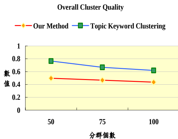
圖 13: Overall Cluster Quality 數值之比較
