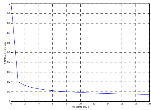
Fig. 4 The PAPR reduction in the proposed scheme
