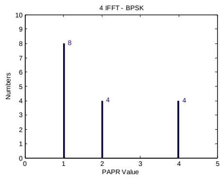
Fig. 3 The histogram of PAPR in the 4-IFFT BPSK OFDM system
