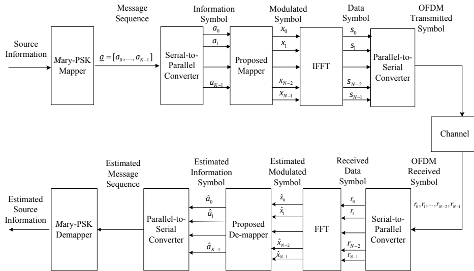
Fig.1 The block diagram of the FFT-based OFDM system
