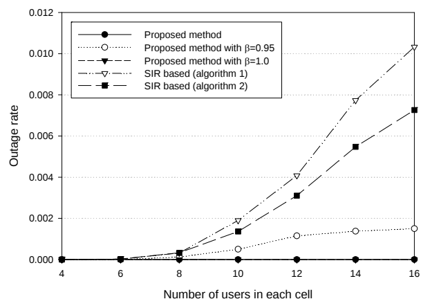
Fig. 3. Outage rate comparison between proposed CCAC method, SIR-based methods [6] and proposed norm approximation method for CDMA cellular system.
