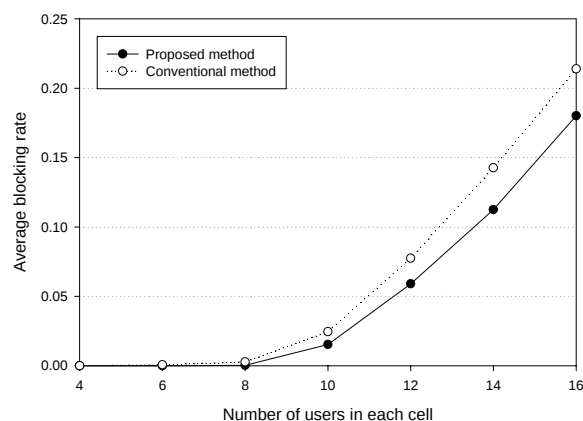
Fig. 4. Average blocking rate comparison between proposed CCAC method and conventional CAC method [8] for multimedia CDMA cellular system
