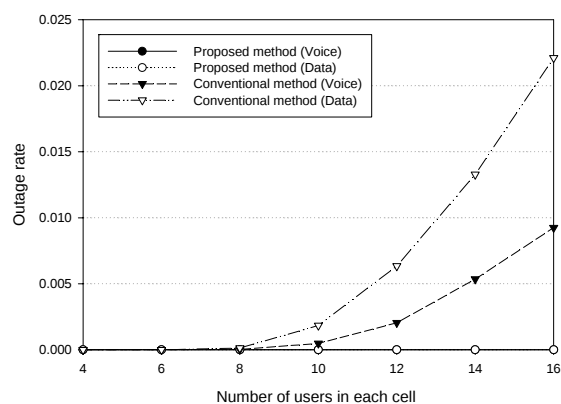
Fig. 5. Outage rate comparison between proposed CCAC method and conventional CAC method [8] for multimedia CDMA cellular system.
