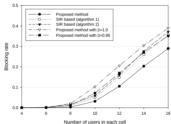
Fig. 2. Blocking rate comparison between proposed CCAC method, SIR-based methods [6] and proposed norm approximation method for CDMA cellular system.
